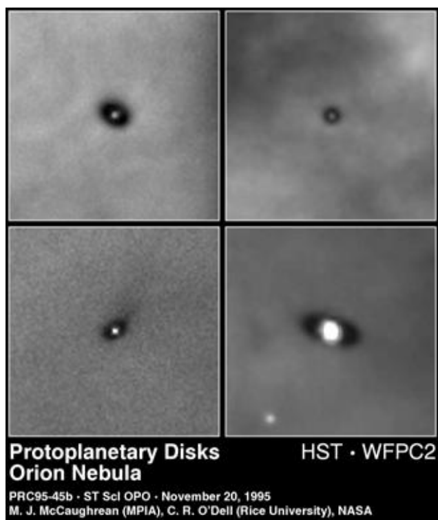
Fig. 2 Four protoplanetary disks and their central stars in front of a bright region in Orion. Permission to reproduce the figure has been granted by ST Sci and by the author, C. R. O'Dell (currently at Vanderbilt University). Taken from web site http://opposite.stsci.edu/pubinfo/jpeg/OriProp4.jpg
