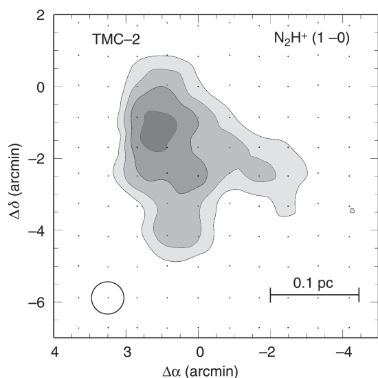
Fig. 3 A contour map of the TMC-2 core in the Taurus molecular cloud as measured via the J = 1 \rightarrow 0 rotational transition of the polar ion \text{N}_2\text{H}^+ . The abscissa and ordinate are in units of minutes of arc along the sky. See text for more details. The author is kindly indebted to his collaborator Paola Caselli (Arcetri Observatory, Florence, Italy) for the figure.
